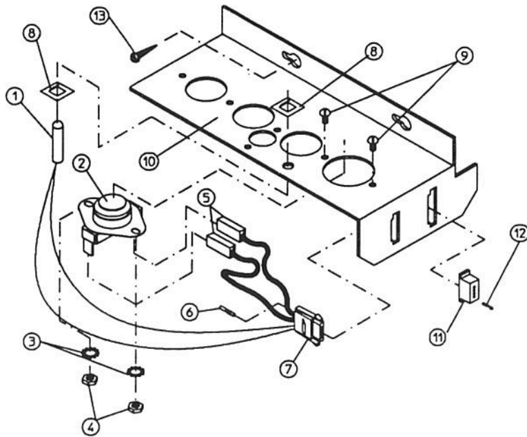
MICROPROCESSOR SENSOR BRACKET ASSEMBLY
