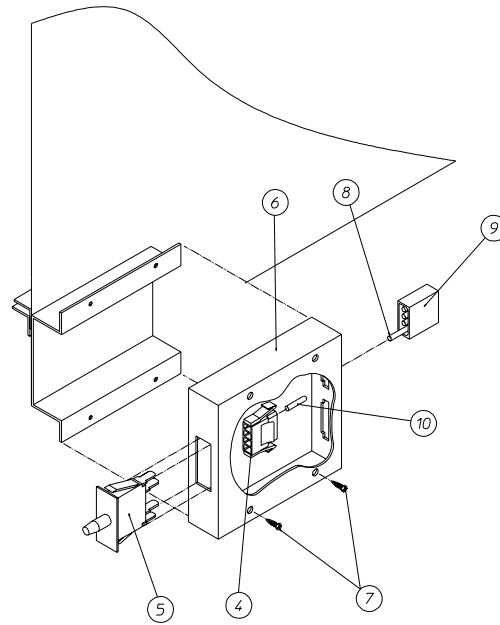
LINT DRAWER SWITCH ASSY
